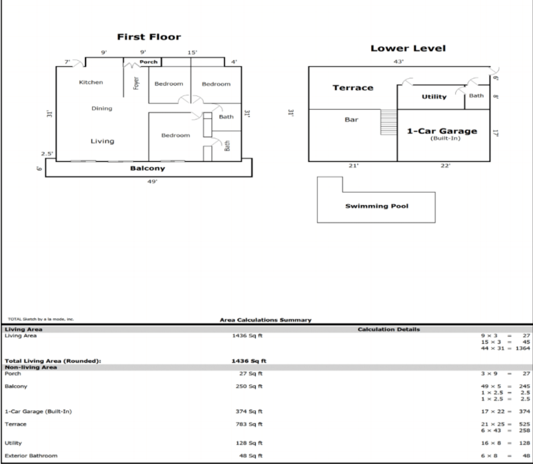
Building Sketch
